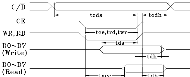
Fig.8-2 Signal timing
